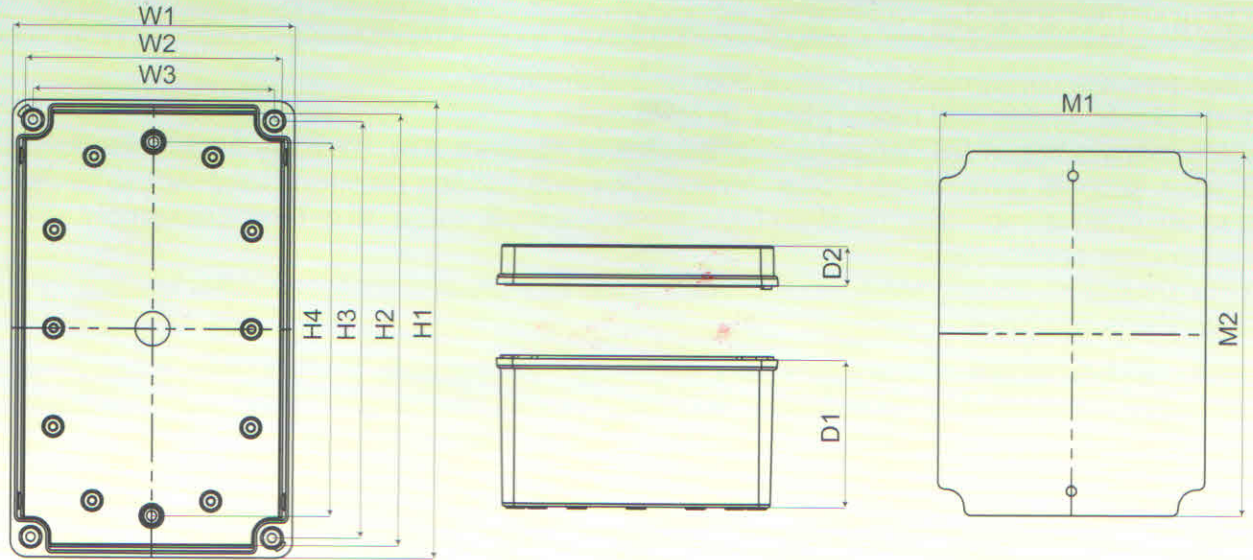
Dimensions (mm)
